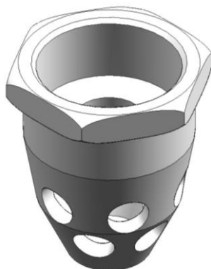
Nozzle 360°
